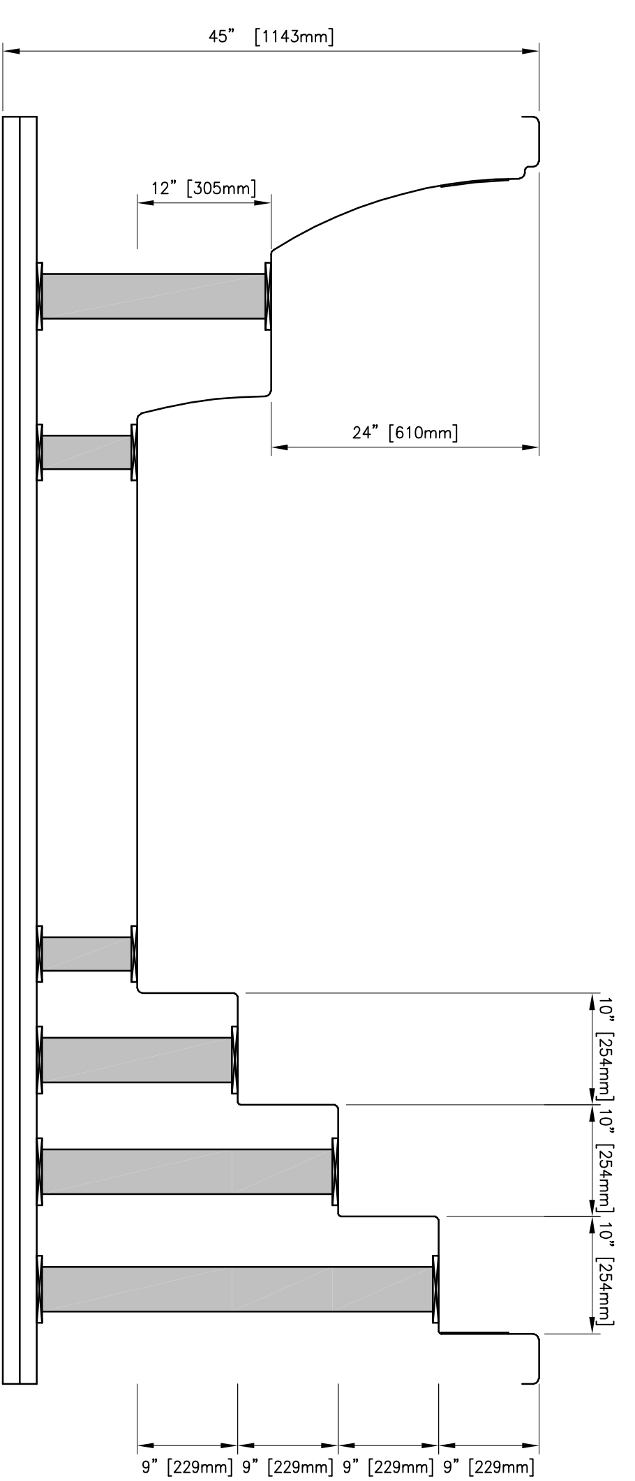
SECTION VIEW—SPA
