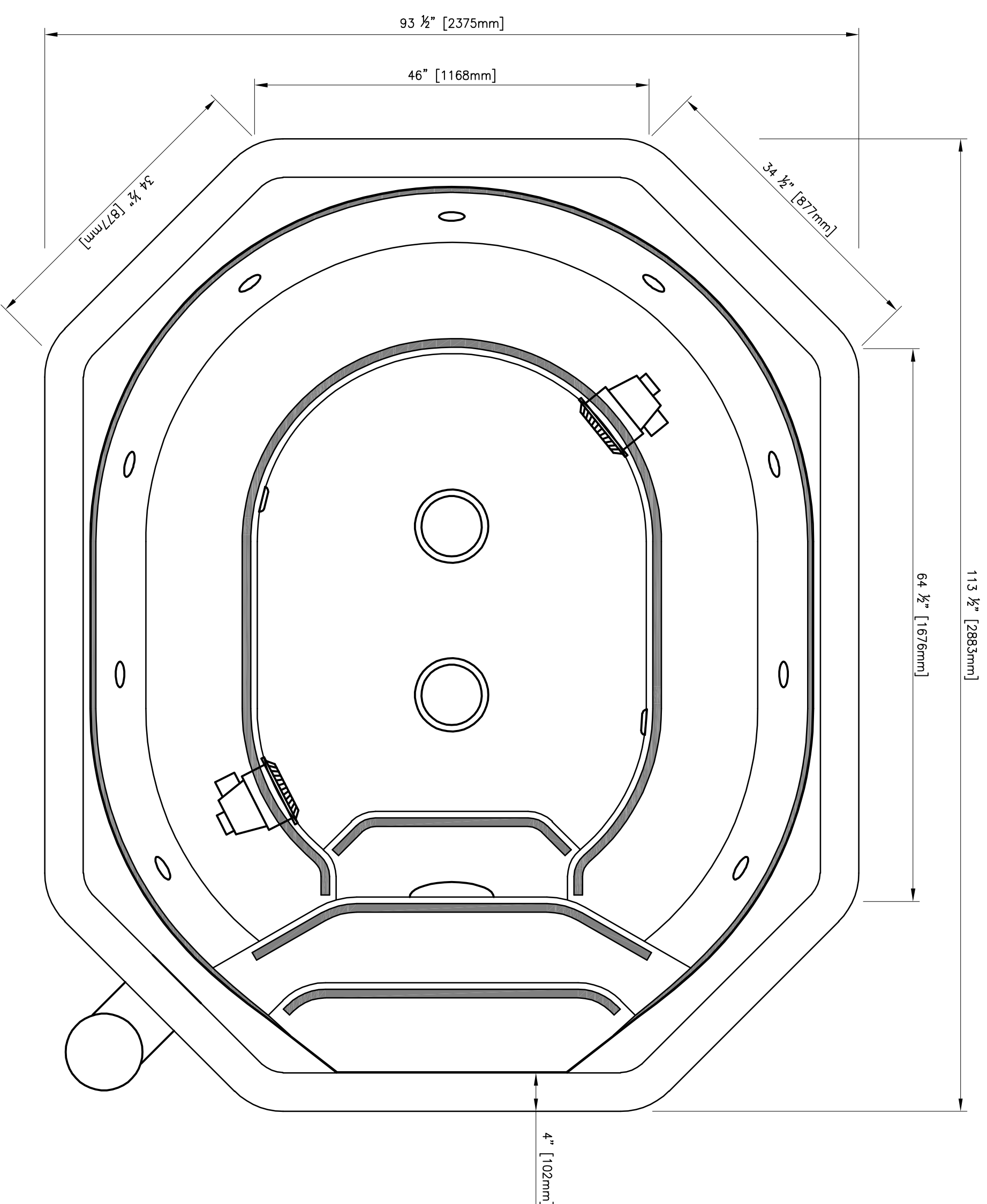
PLAN VIEW—SPA
